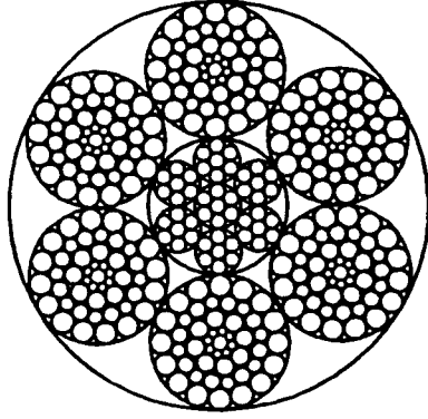
6x49 SWS (16-8+8-8-1) (CWR) 48 to 92 mm
