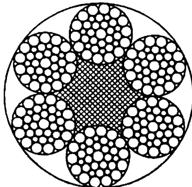
6x36 SW (14-7+7-7-1) (CF) 13 to 56 mm
